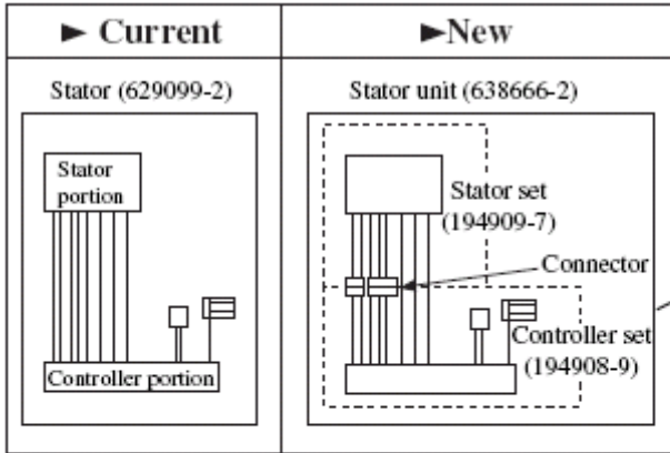
Circuit diagram including new Stator unit
