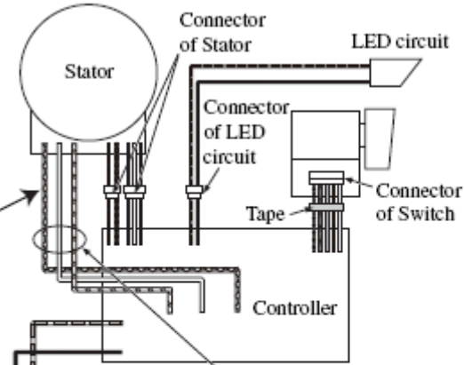
Circuit diagram including new Stator unit
